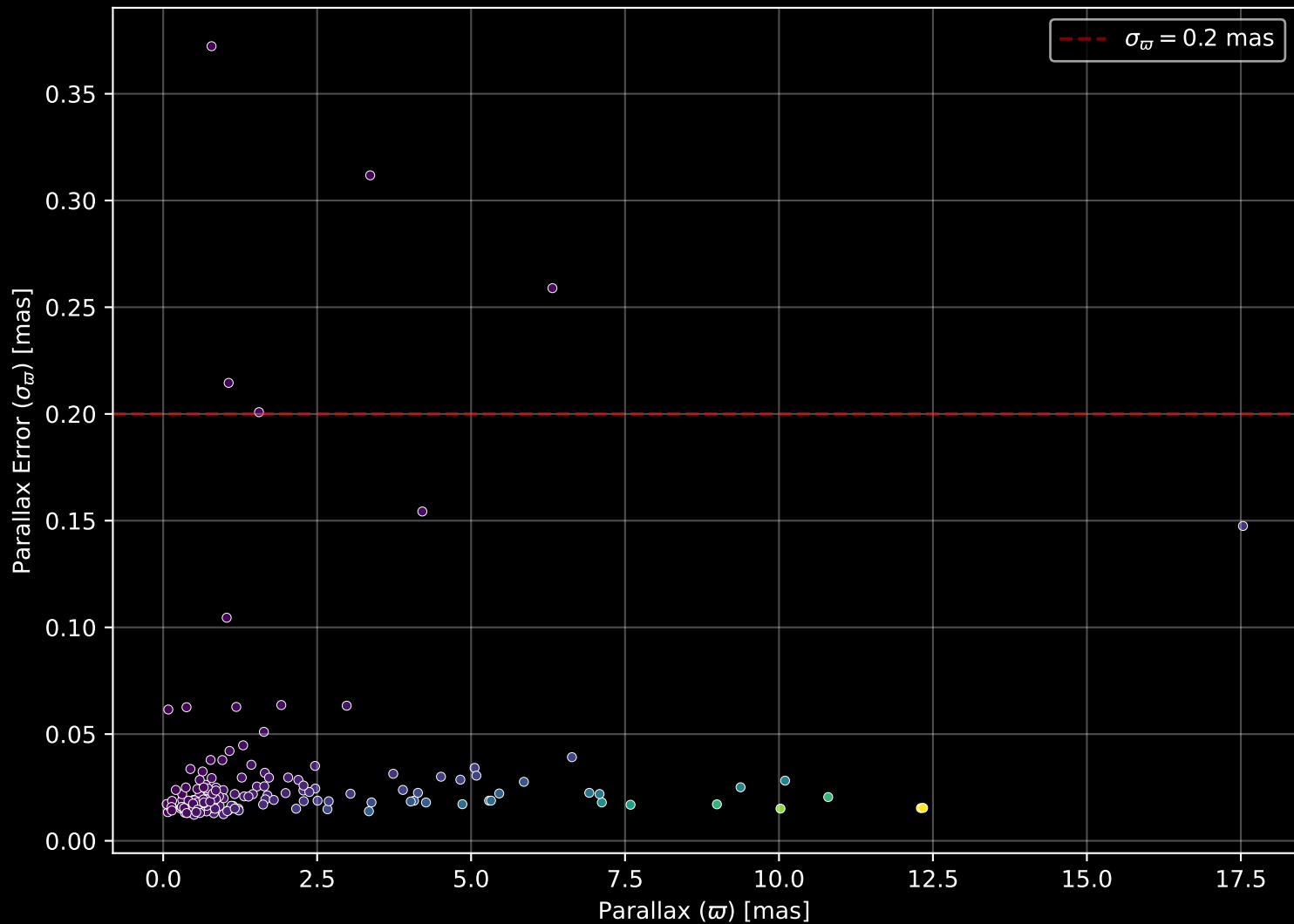
APOGEE DR17 Field: [191+24_MGA] Parallax Quality (n= 173)
