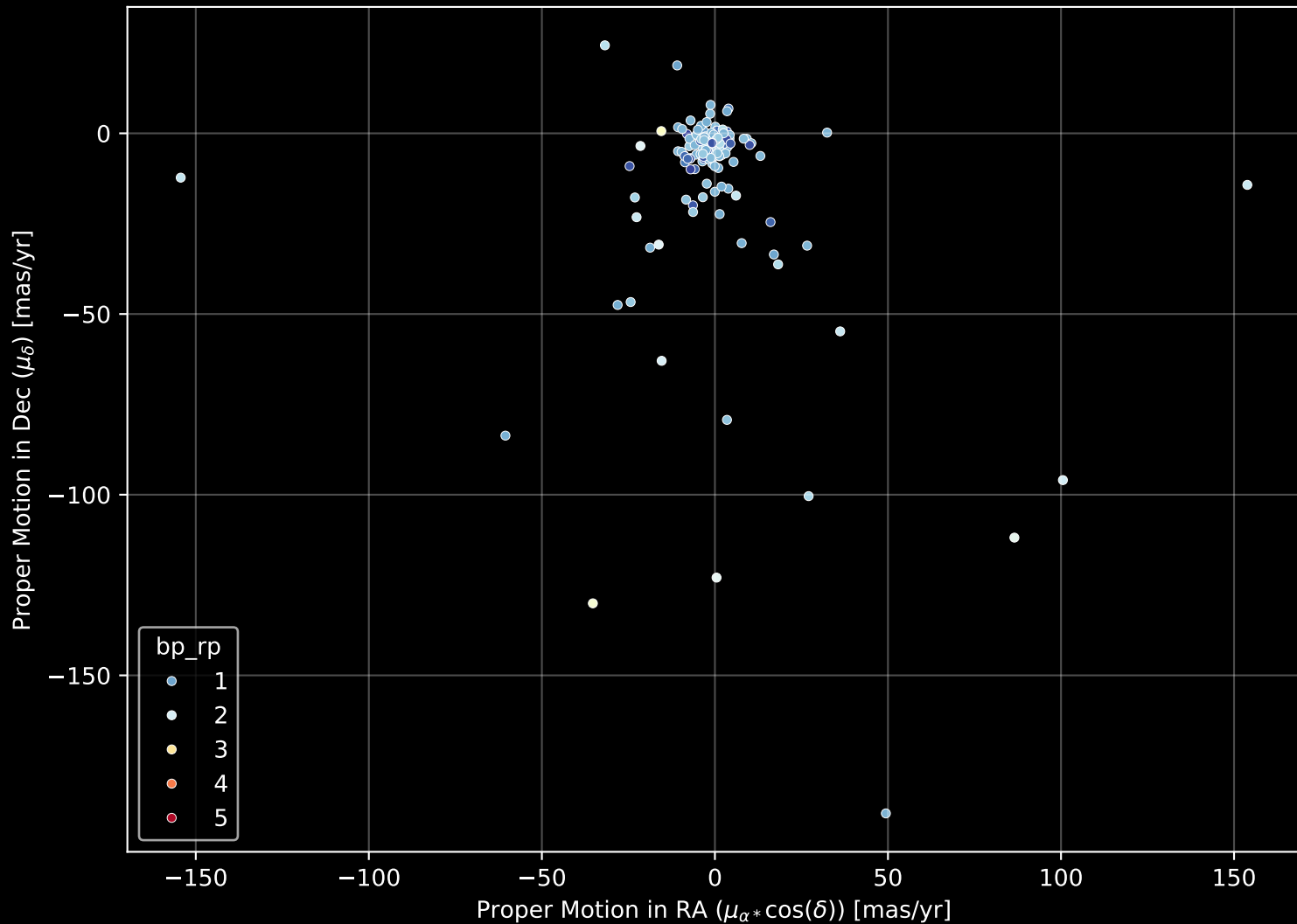
APOGEE DR17 Field: [191+24_MGA] Proper Motion Diagram (n= 173)
