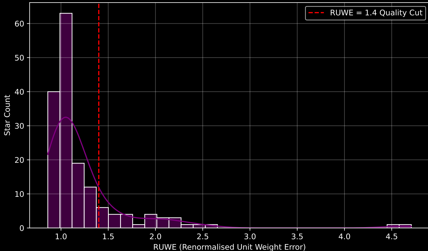
GAPOGEE DR17 Field [191+24_MGA] RUWE Distribution (n= 164)
