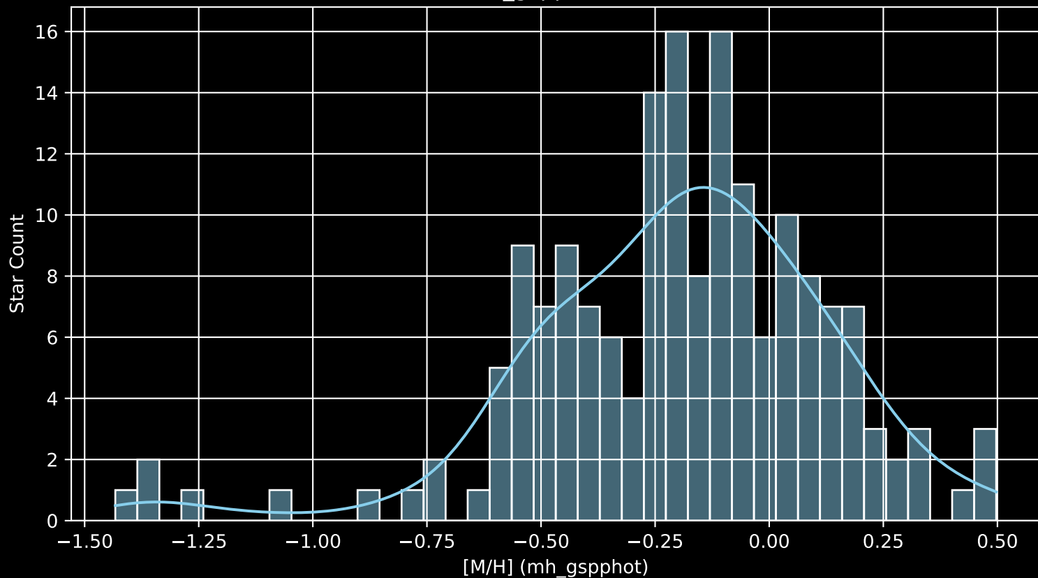
APOGEE DR17 Field: [191+24_MGA [M/H] (mh_gspphot) (n= 172)
