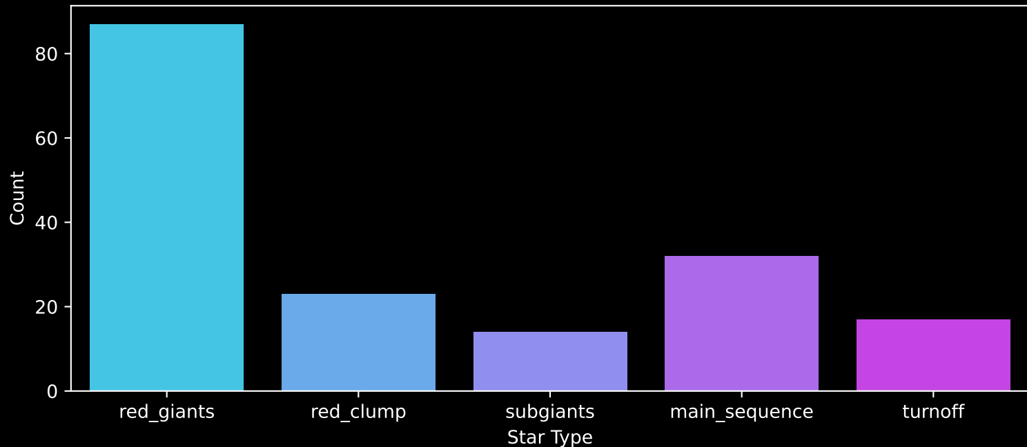
APOGEE DR17 Field: [191+24_MGA] Count plot of Star Type
